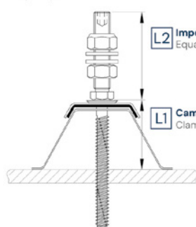
Profilo trapezoidale ed elemento sandwich Trapeze profile and sandwich element
