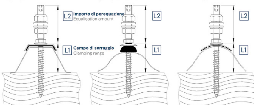
Profilo trapezoidale ed elemento sandwich Trapeze profile and sandwich element
