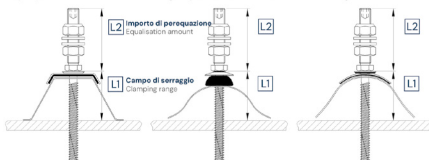
Profilo trapezoidale ed elemento sandwich Trapeze profile and sandwich element
