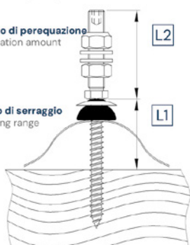
Profilo trapezoidale ed elemento sandwich Trapeze profile and sandwich element
