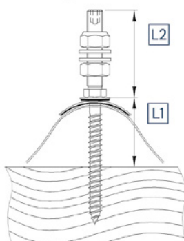
Fibrocemento ondulato Corrugated fibre cement
