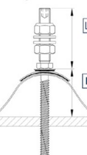
Ciment ondulé Corrugated fibre cement
