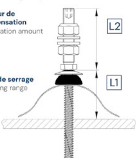
Profilé ondulé et élément sandwich Corrugated profile and sandwich element
