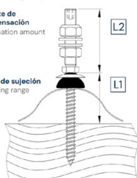
Perfil ondulado y elemento sandwich Corrugated profile and sandwich element
