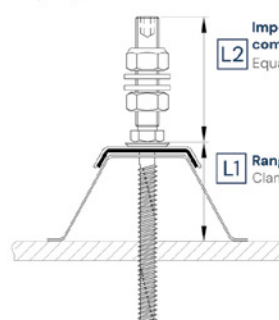
Perfil trapezoidal y elemento sándwich Trapeze profile and sandwich element
