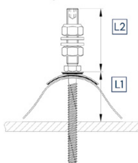
Fibrocemento ondulado Corrugated fibre cement
