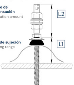
Perfil ondulado y elemento sándwich Corrugated profile and sandwich element
