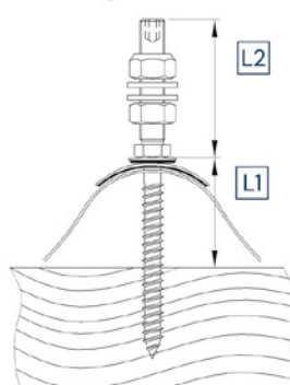
Fibrocemento ondulado Corrugated fibre cement
