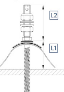
Fibrocemento ondulado Corrugated fibre cement
