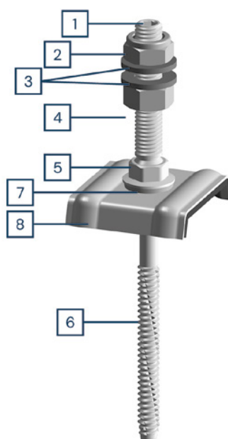
Perfil trapezoidal y elemento sándwich Trapeze profile and sandwich element
