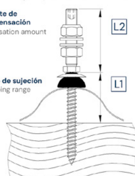
Perfil ondulado y elemento sándwich Corrugated profile and sandwich element
